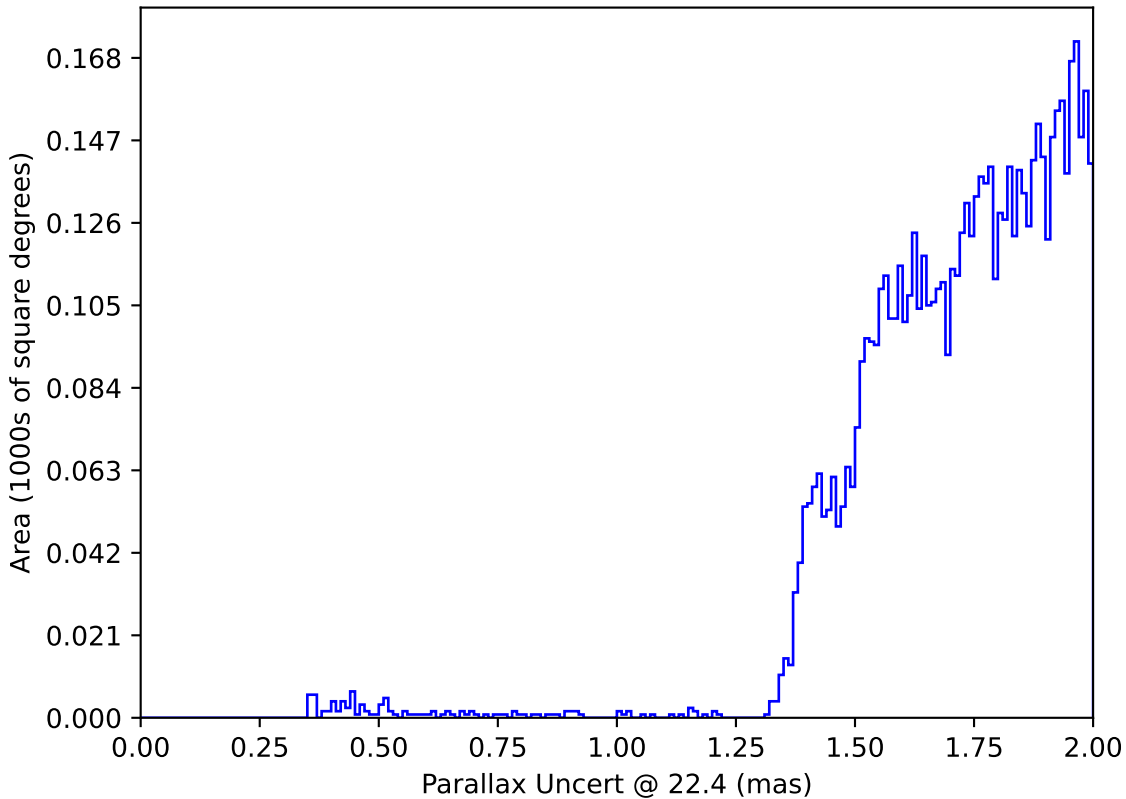
roll_pause_mjdp60_v3.4_10yrs : Parallax Uncert @ 22.4
