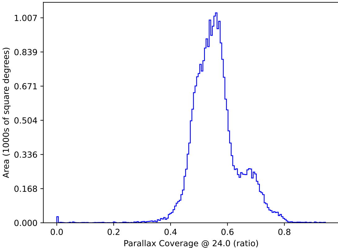
roll_pause_mjdp60_v3.4_10yrs : Parallax Coverage @ 24.0
