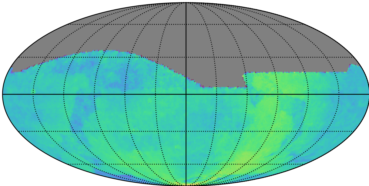
roll_pause_mjdp60_v3.4_10yrs : Parallax Coverage @ 22.4
