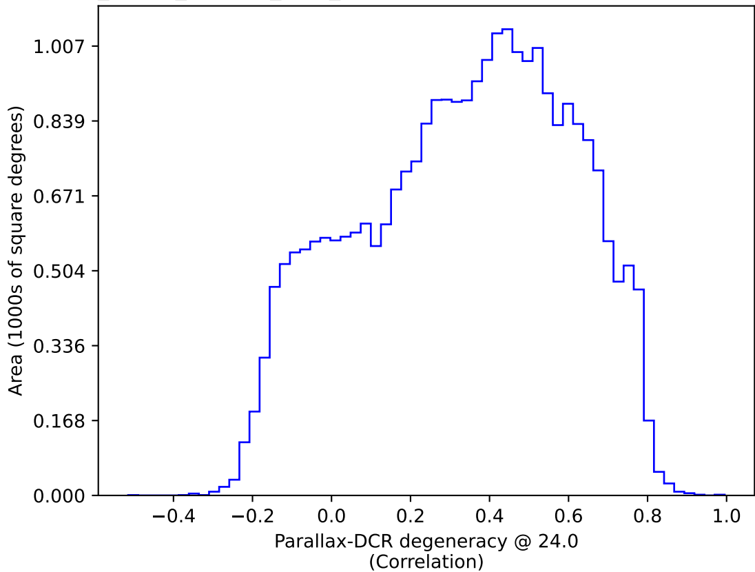
roll_pause_mjdp60_v3.4_10yrs : Parallax-DCR degeneracy @ 24.0
