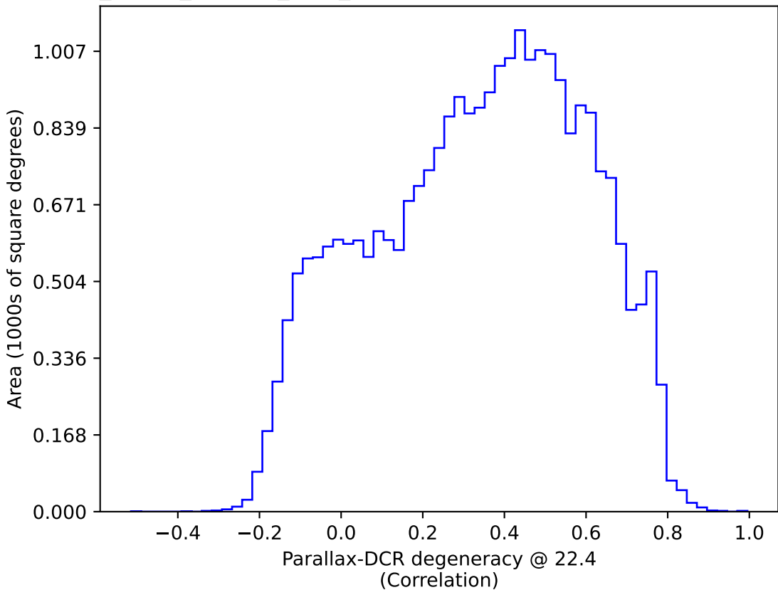
roll_pause_mjdp60_v3.4_10yrs : Parallax-DCR degeneracy @ 22.4
