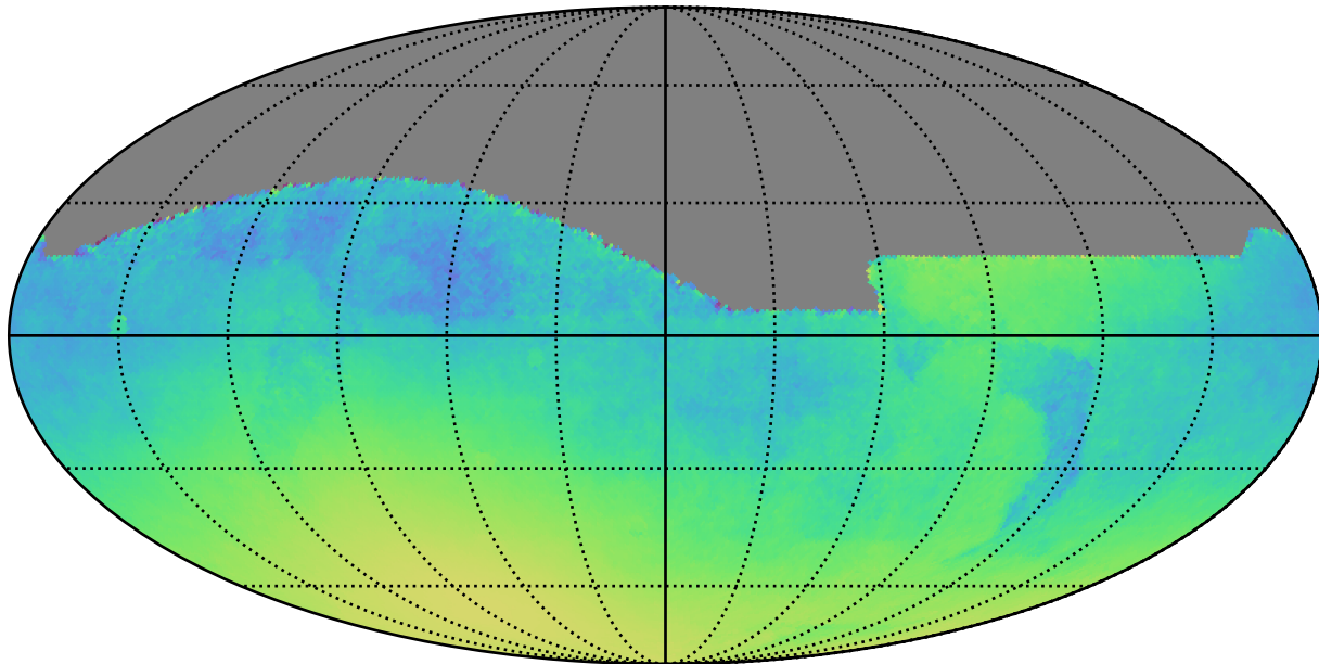
roll_pause_mjdp60_v3.4_10yrs : Normalized Parallax Uncert @ 24.0
