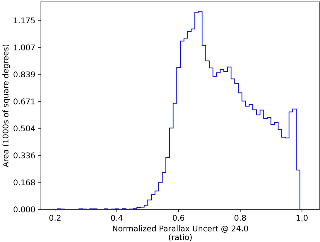
roll_pause_mjdp60_v3.4_10yrs : Normalized Parallax Uncert @ 24.0
