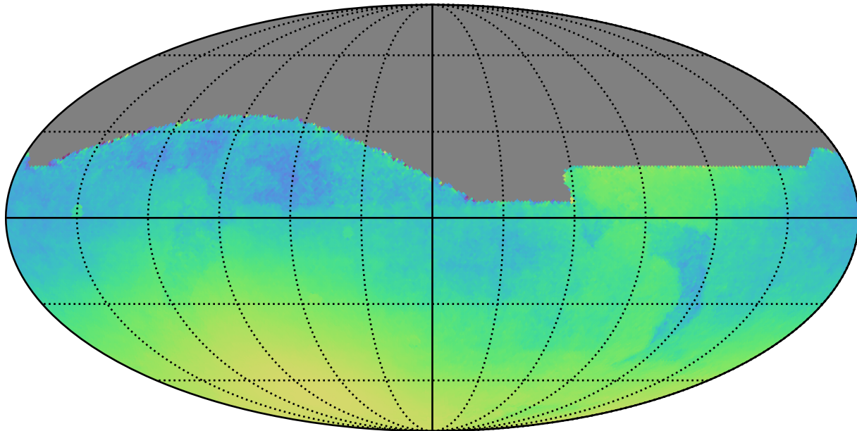
roll_pause_mjdp60_v3.4_10yrs : Normalized Parallax Uncert @ 22.4
