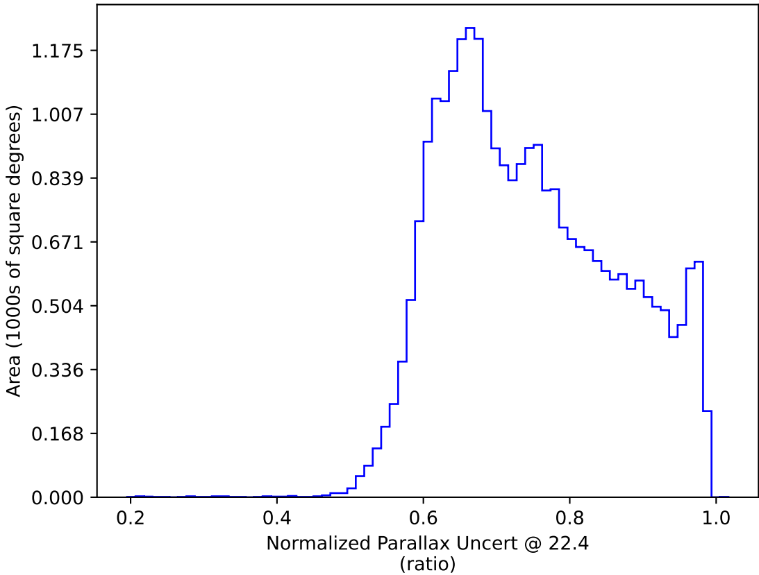
roll_pause_mjdp60_v3.4_10yrs : Normalized Parallax Uncert @ 22.4
