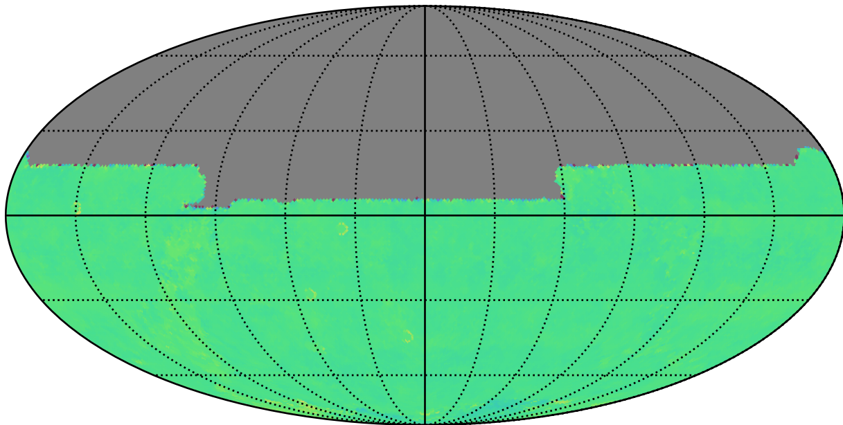
roll_pause_mjdp60_v3.4_10yrs y: Kuiper rotTelPos
