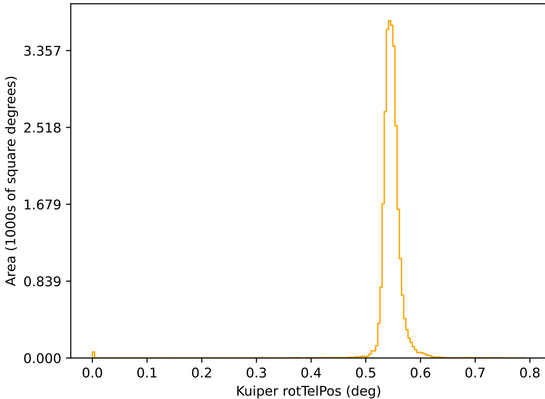
roll_pause_mjdp60_v3.4_10yrs r: Kuiper rotTelPos
