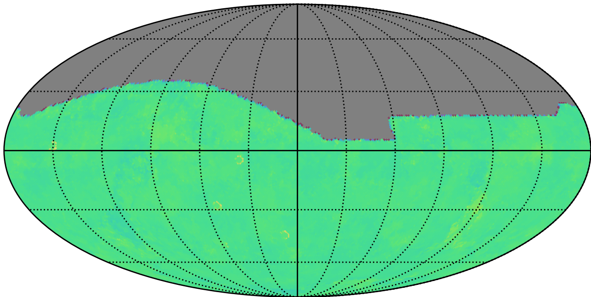
roll_pause_mjdp60_v3.4_10yrs g: Kuiper rotTelPos
