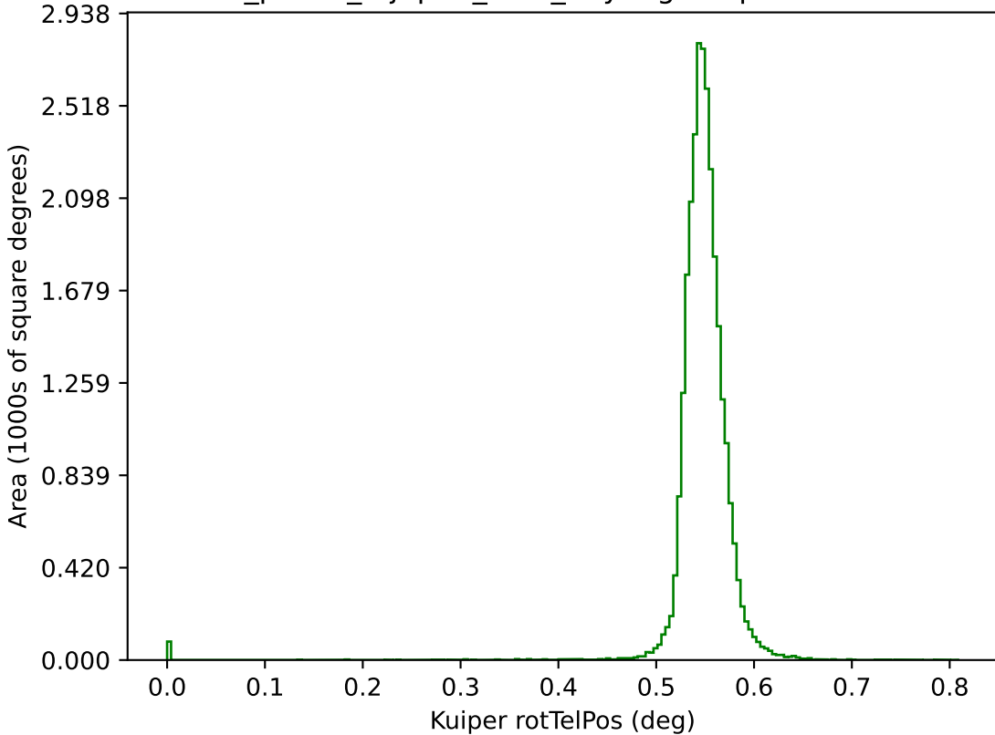
roll_pause_mjdp60_v3.4_10yrs g: Kuiper rotTelPos
