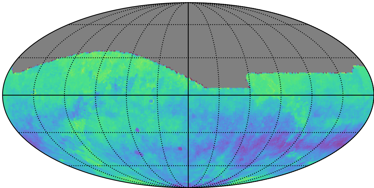
roll_pause_mjdp60_v3.4_10yrs z: Kuiper rotSkyPos
