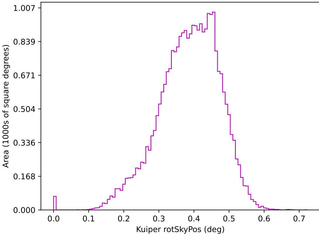
roll_pause_mjdp60_v3.4_10yrs z: Kuiper rotSkyPos
