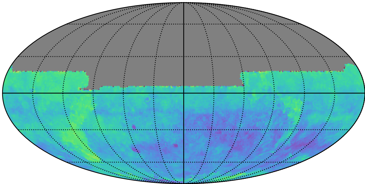
roll_pause_mjdp60_v3.4_10yrs y: Kuiper rotSkyPos
