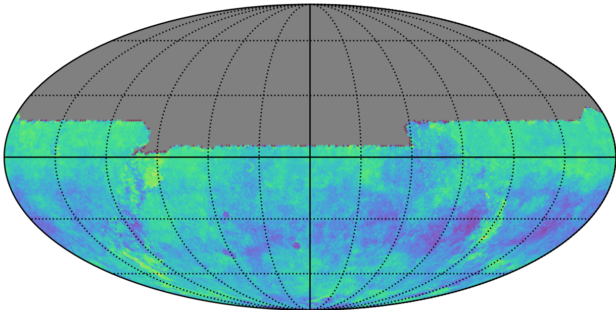
roll_pause_mjdp60_v3.4_10yrs u: Kuiper rotSkyPos
