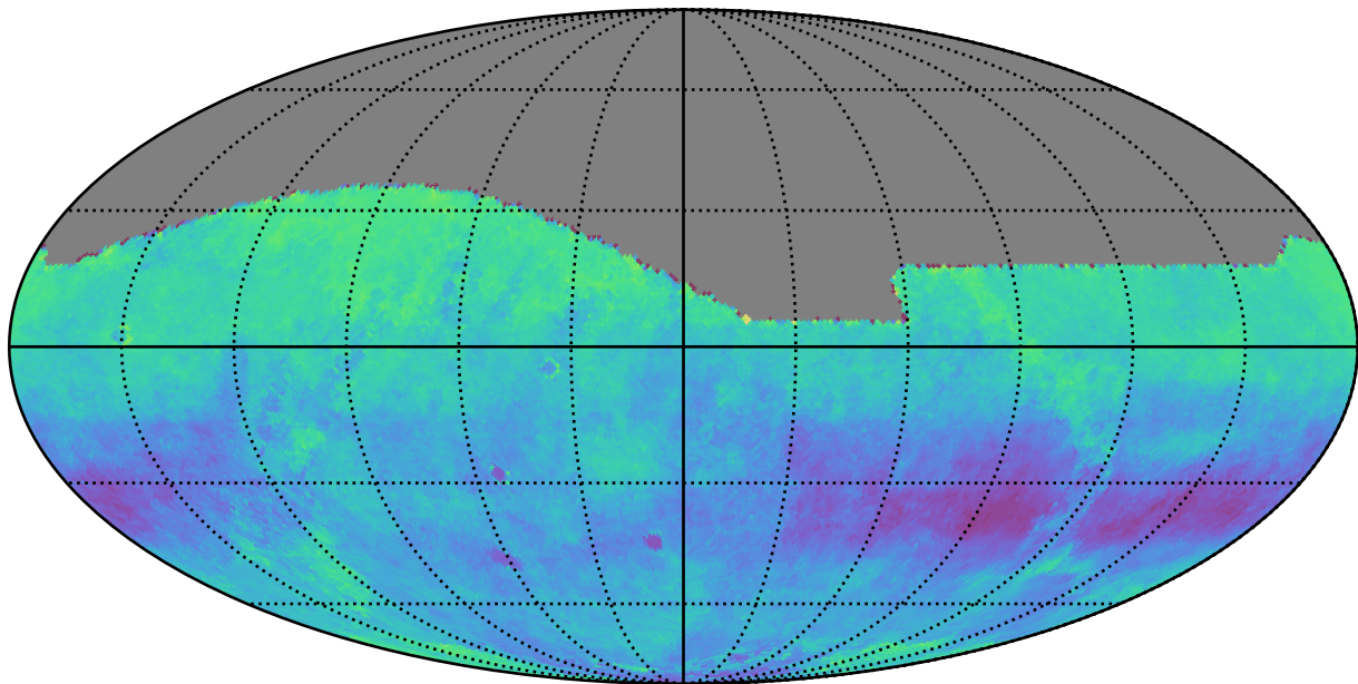
roll_pause_mjdp60_v3.4_10yrs r: Kuiper rotSkyPos
