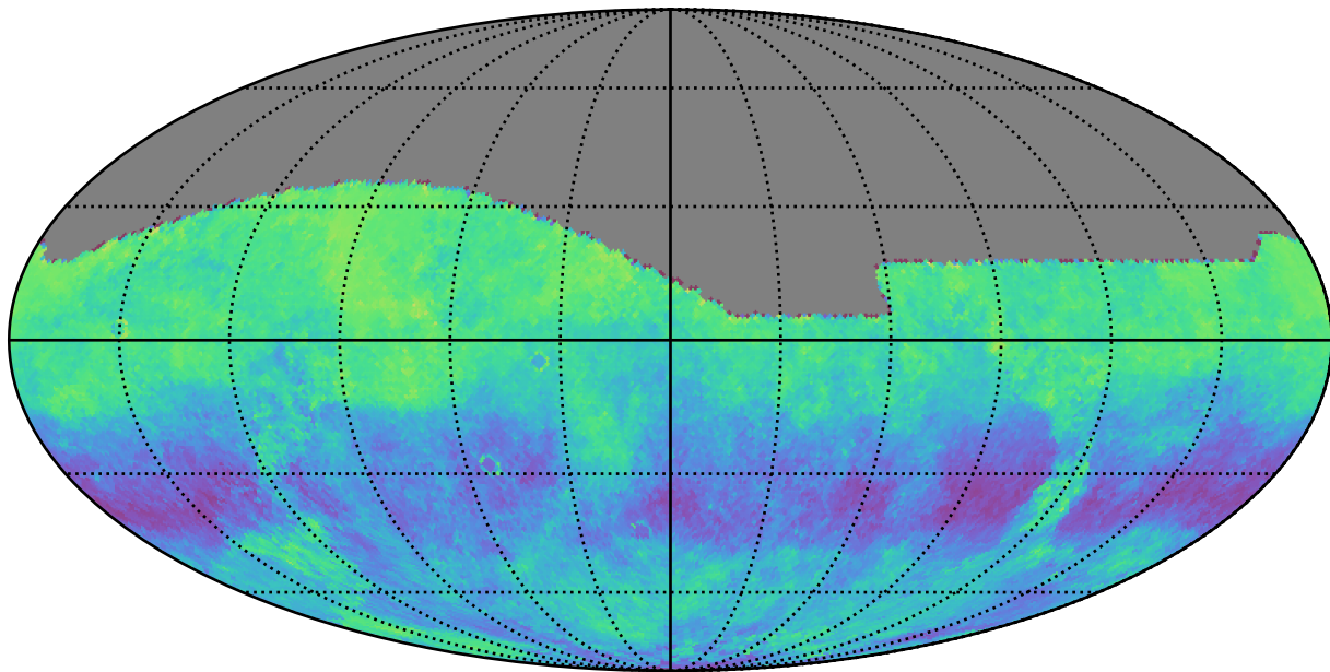
roll_pause_mjdp60_v3.4_10yrs g: Kuiper rotSkyPos
