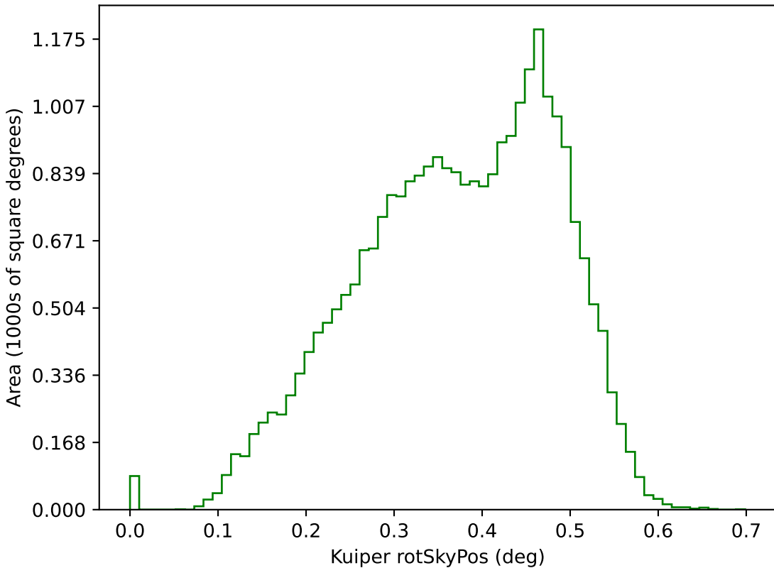
roll_pause_mjdp60_v3.4_10yrs g: Kuiper rotSkyPos
