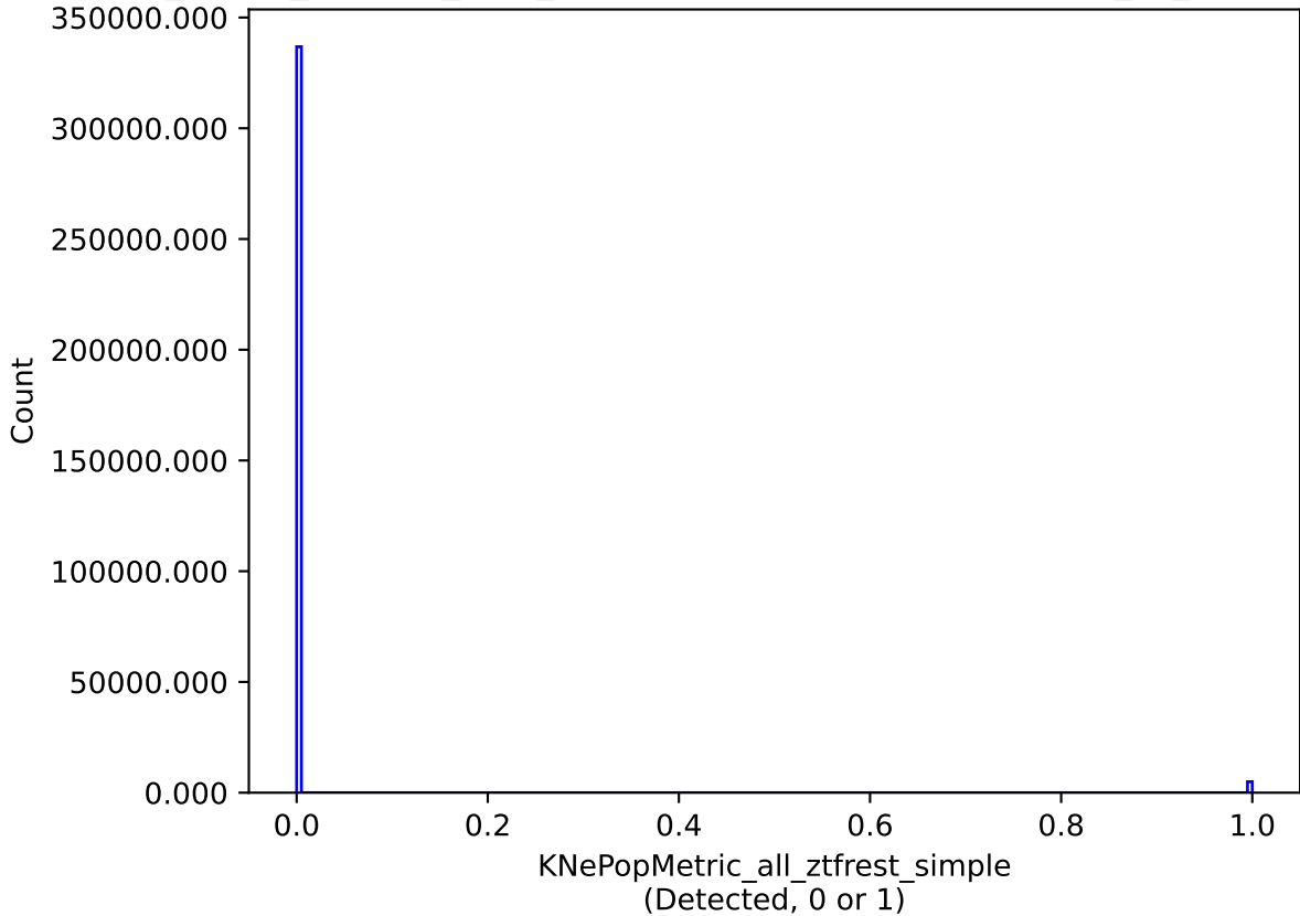
roll_pause_mjdp60_v3.4_10yrs all models: KNePopMetric_all_ztfrest_simple
