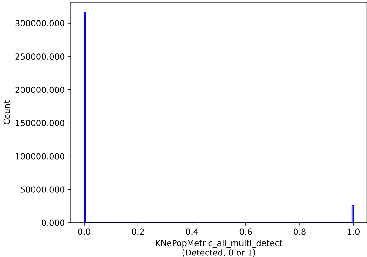
roll_pause_mjdp60_v3.4_10yrs all models: KNePopMetric_all_multi_detect
