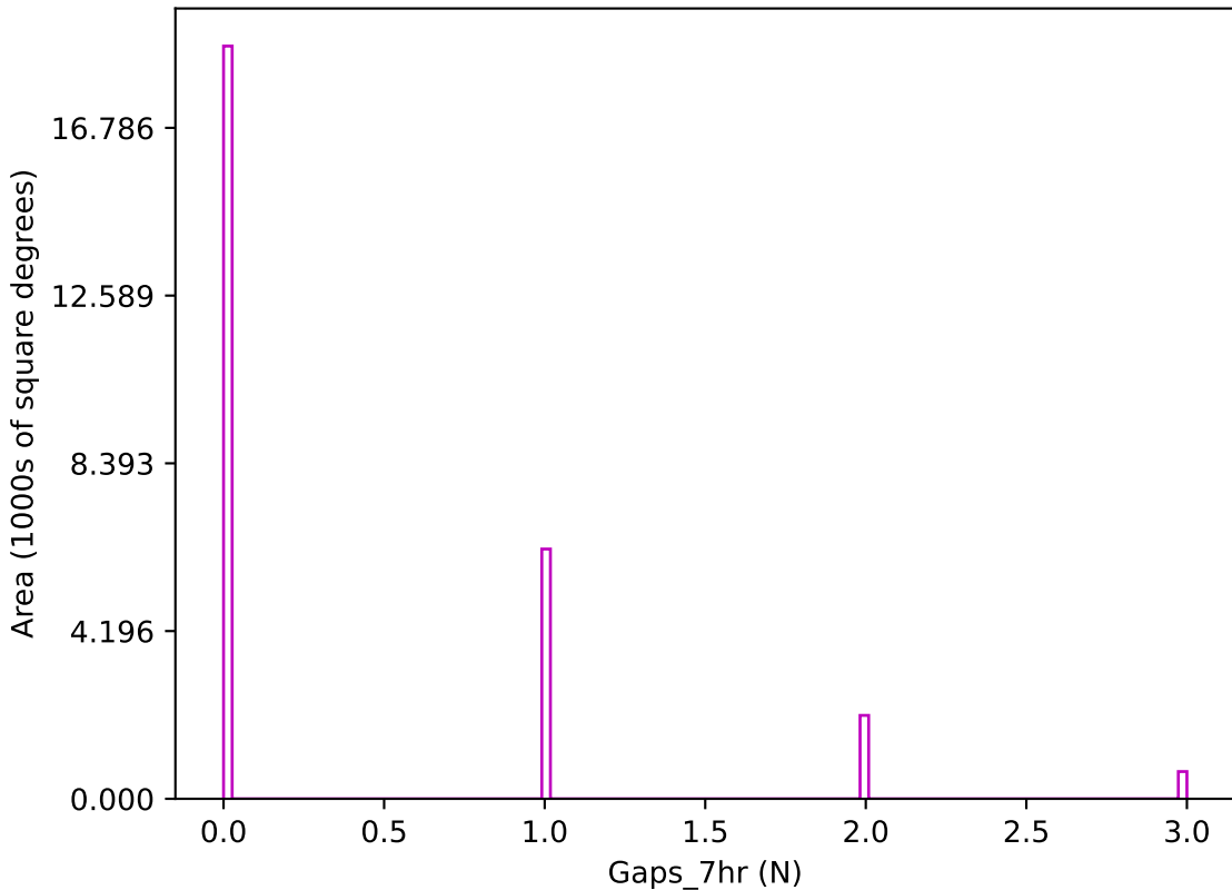
roll_pause_mjdp60_v3.4_10yrs z band: Gaps_7hr
