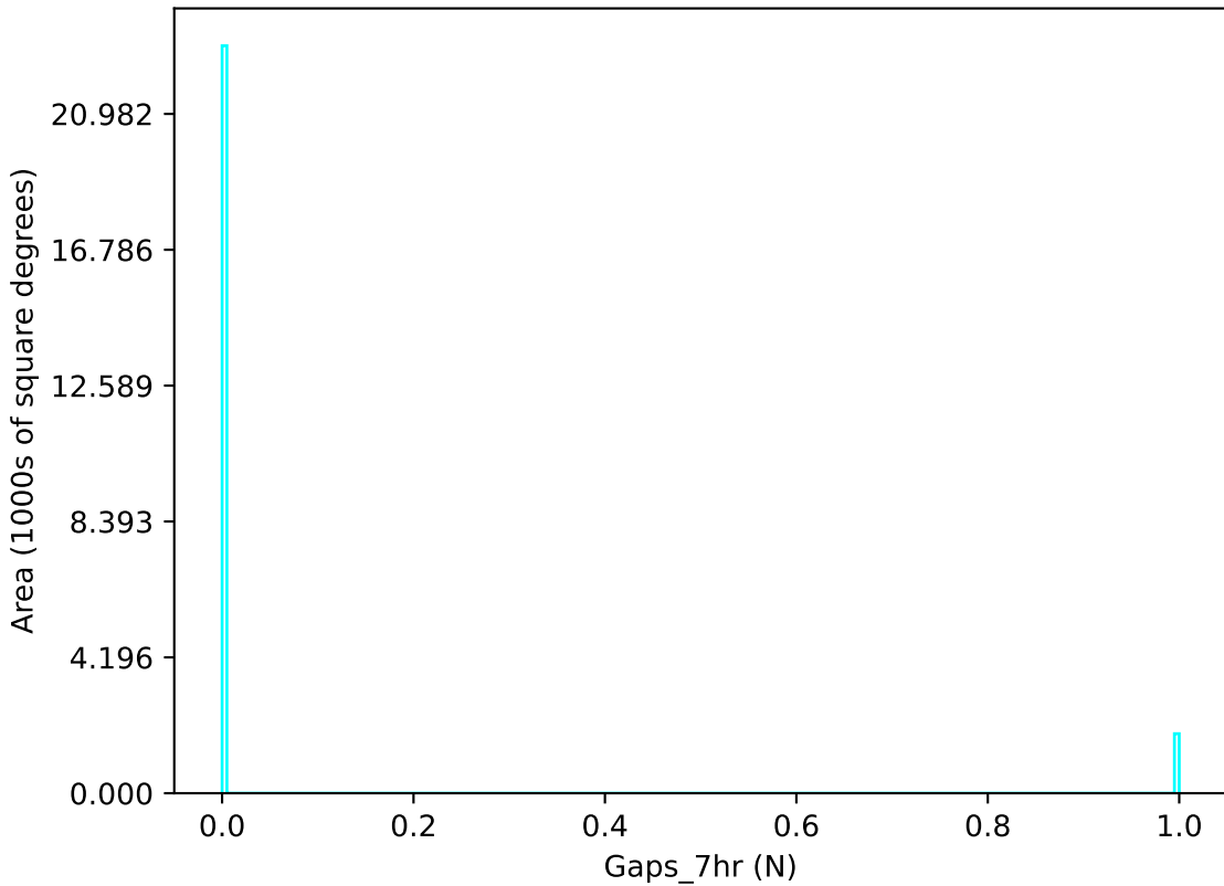
roll_pause_mjdp60_v3.4_10yrs u band: Gaps_7hr
