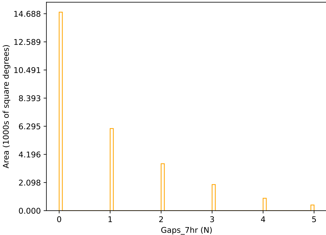
roll_pause_mjdp60_v3.4_10yrs r band: Gaps_7hr
