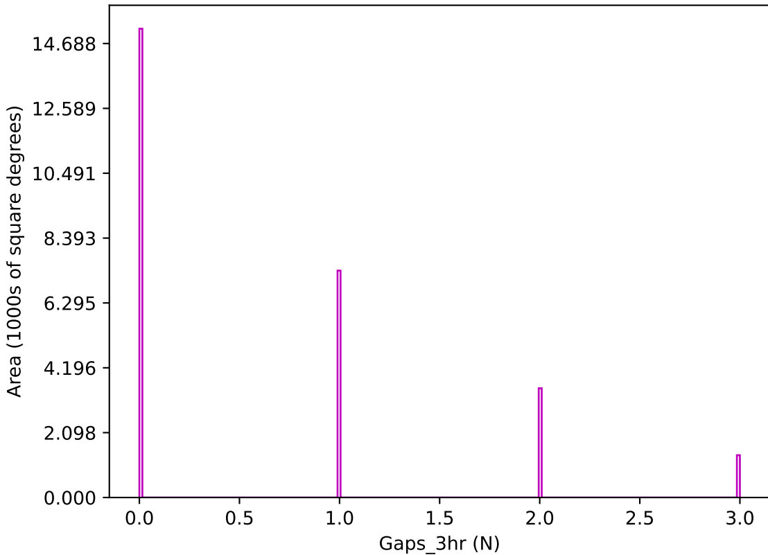
roll_pause_mjdp60_v3.4_10yrs z band: Gaps_3hr
