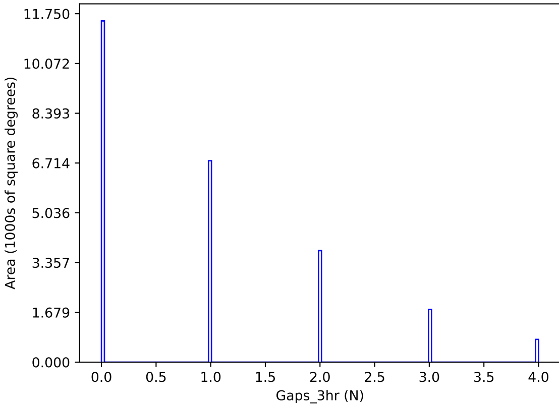
roll_pause_mjdp60_v3.4_10yrs y band: Gaps_3hr
