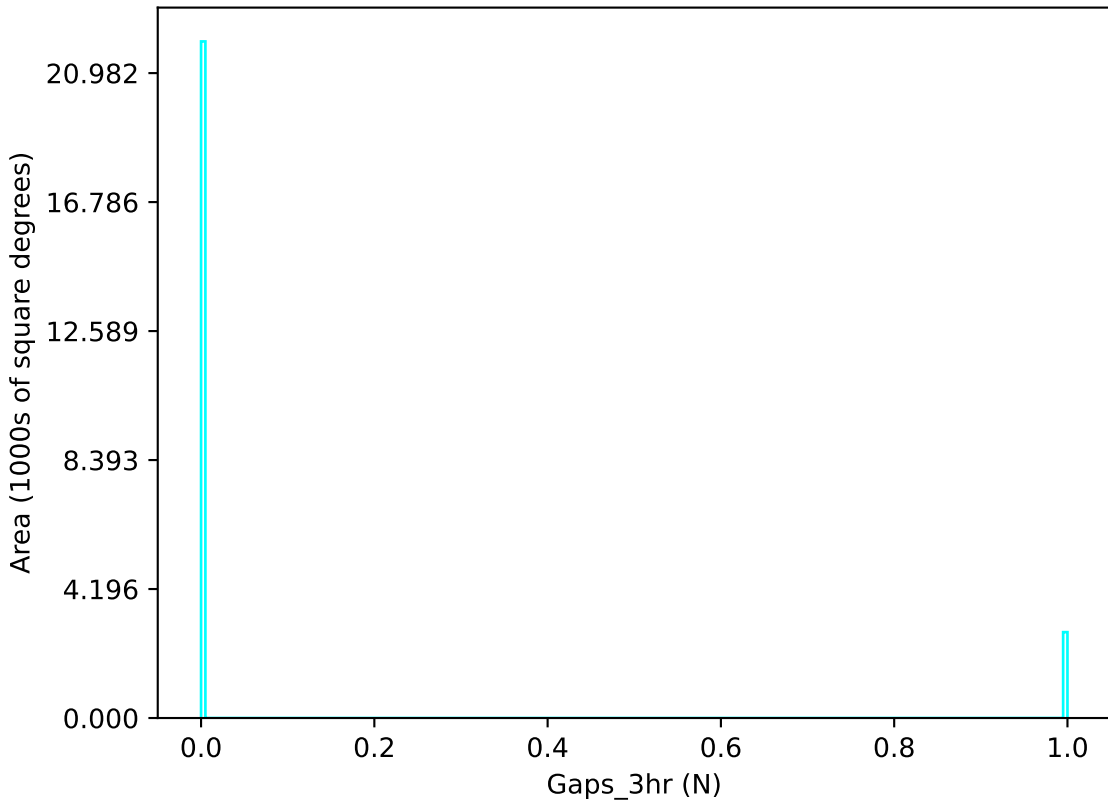
roll_pause_mjdp60_v3.4_10yrs u band: Gaps_3hr
