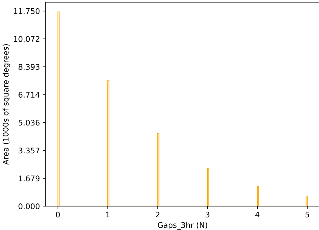
roll_pause_mjdp60_v3.4_10yrs r band: Gaps_3hr
