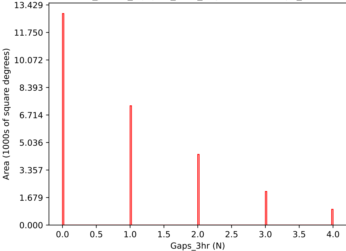
roll_pause_mjdp60_v3.4_10yrs i band: Gaps_3hr
