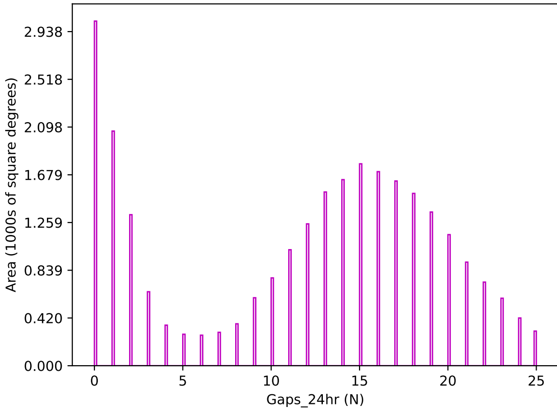
roll_pause_mjdp60_v3.4_10yrs z band: Gaps_24hr
