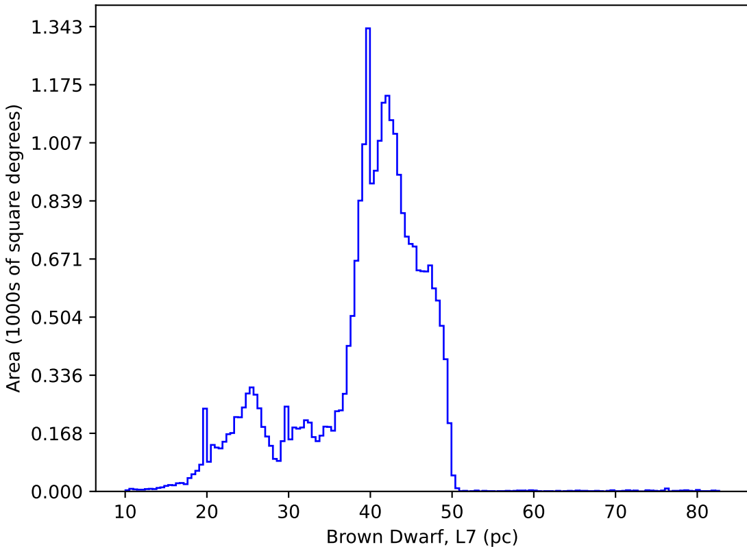
roll_pause_mjdp60_v3.4_10yrs : Brown Dwarf, L7
