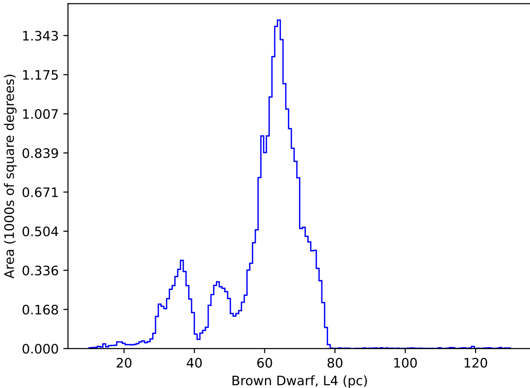
roll_pause_mjdp60_v3.4_10yrs : Brown Dwarf, L4
