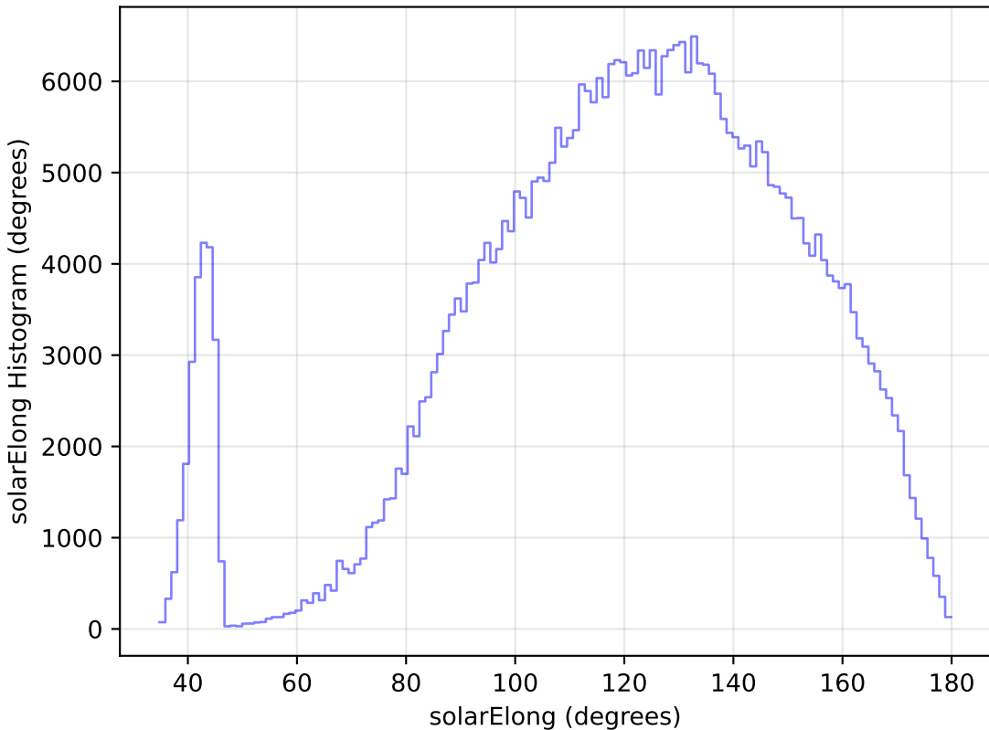
roll_pause_mjdp60_v3.4_10yrs WFD z band: solarElong Histogram
