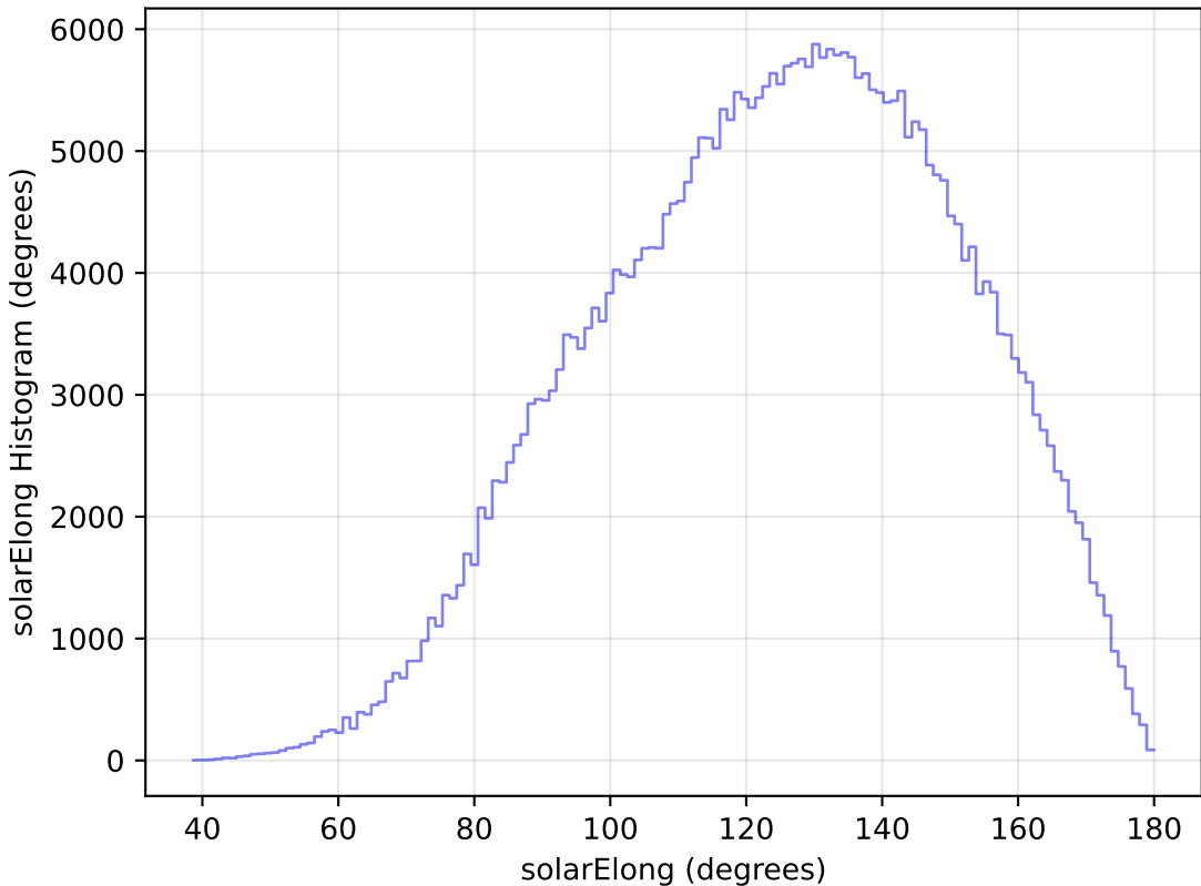
roll_pause_mjdp60_v3.4_10yrs WFD y band: solarElong Histogram
