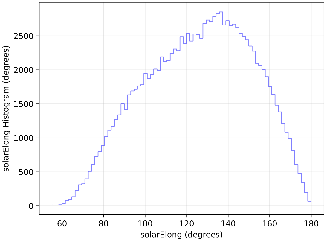
roll_pause_mjdp60_v3.4_10yrs WFD u band: solarElong Histogram
