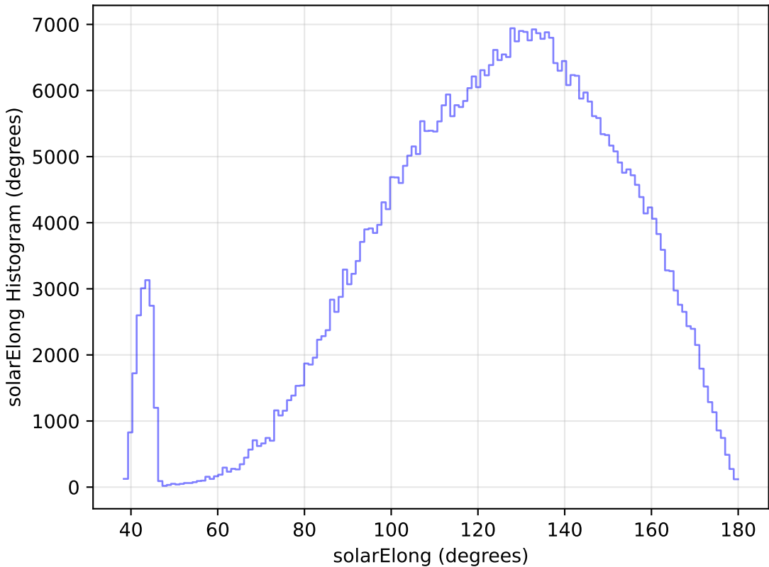
roll_pause_mjdp60_v3.4_10yrs WFD r band: solarElong Histogram
