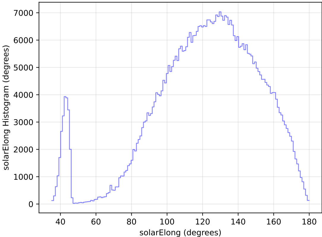
roll_pause_mjdp60_v3.4_10yrs WFD i band: solarElong Histogram
