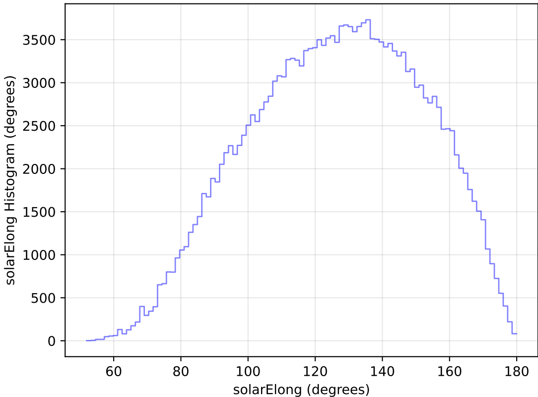
roll_pause_mjdp60_v3.4_10yrs WFD g band: solarElong Histogram
