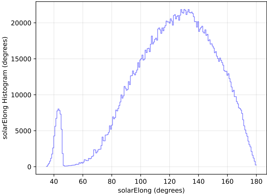
roll_pause_mjdp60_v3.4_10yrs WFD all bands: solarElong Histogram
