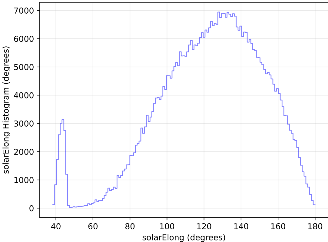
roll_pause_mjdp60_v3.4_10yrs All sky r band: solarElong Histogram
