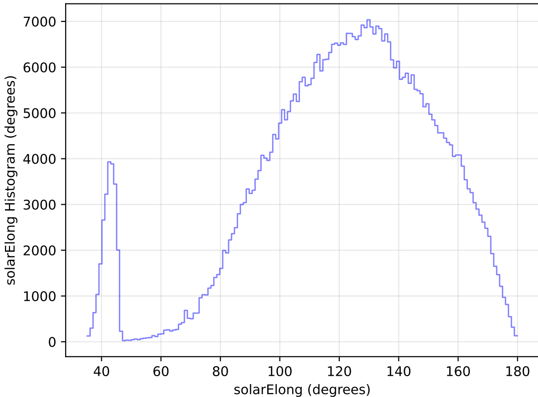
roll_pause_mjdp60_v3.4_10yrs All sky i band: solarElong Histogram
