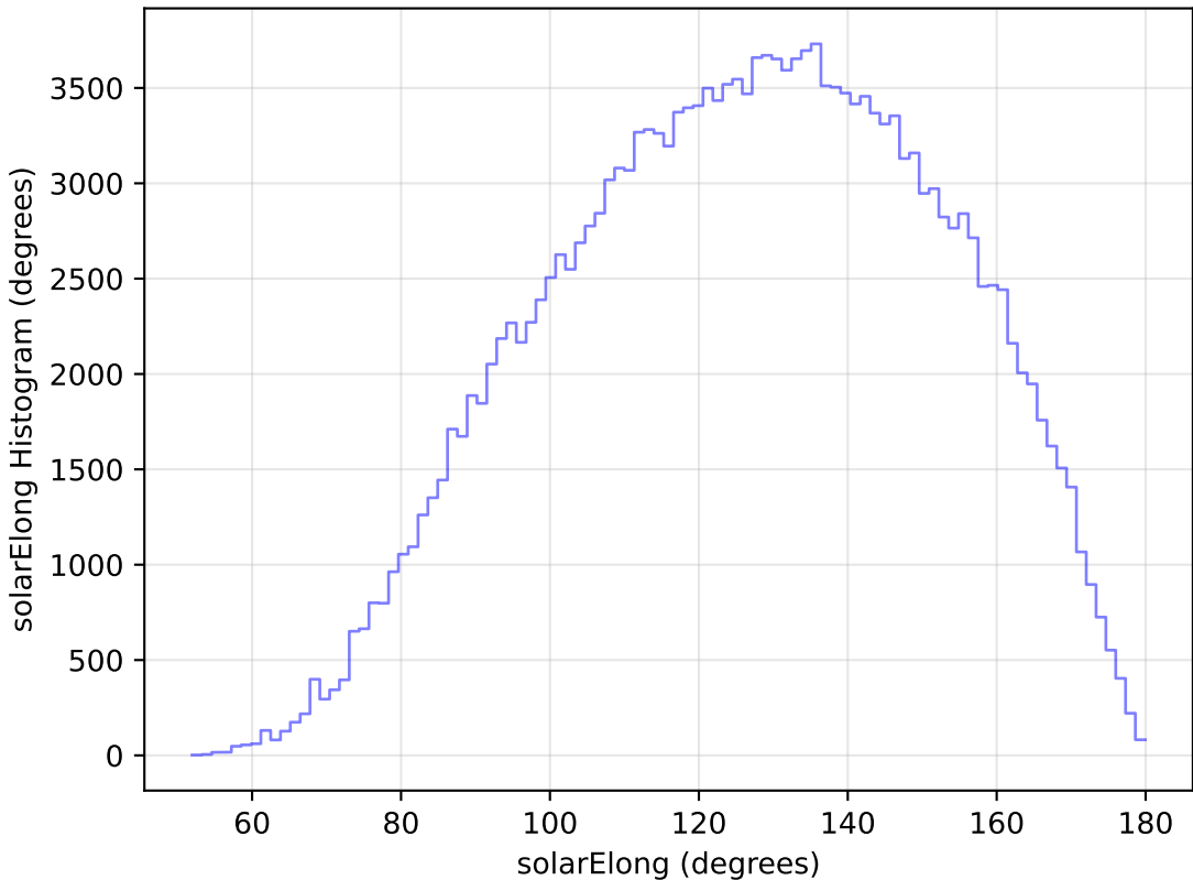
roll_pause_mjdp60_v3.4_10yrs All sky g band: solarElong Histogram
