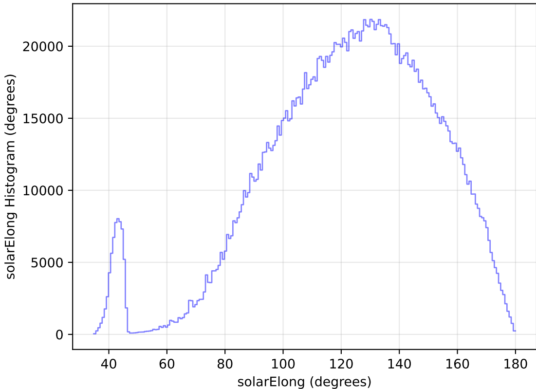
roll_pause_mjdp60_v3.4_10yrs All sky all bands: solarElong Histogram
