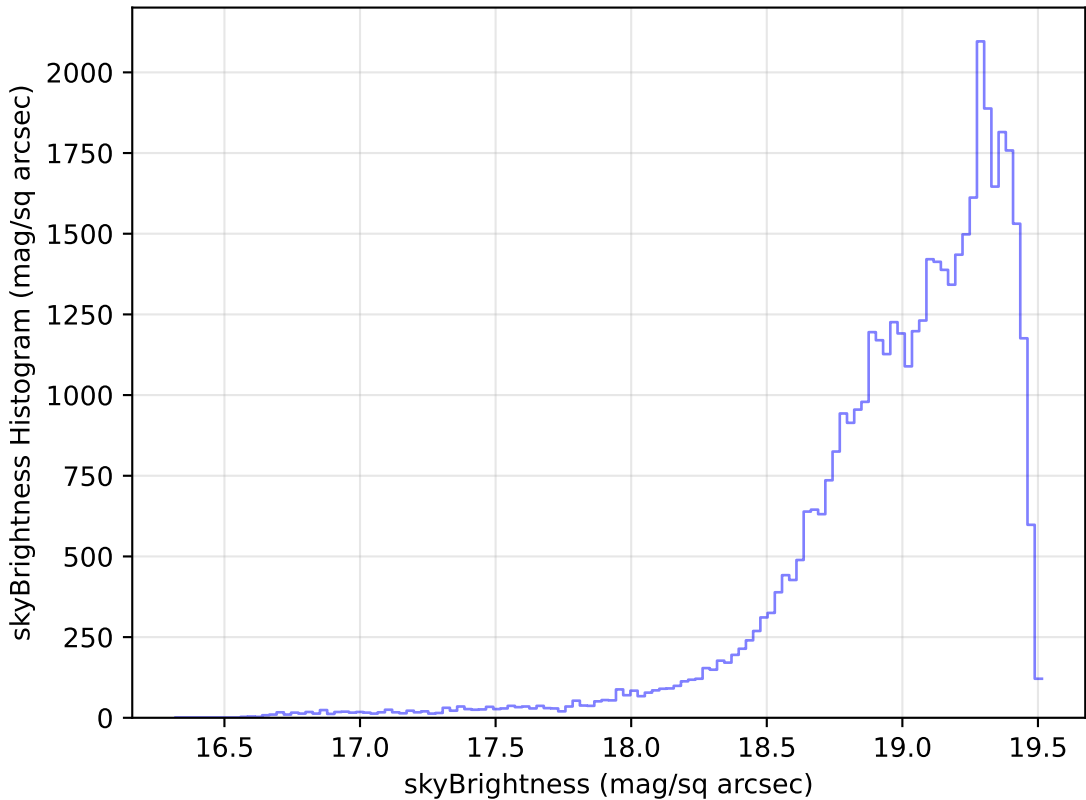
roll_pause_mjdp60_v3.4_10yrs Yr 1 z band: skyBrightness Histogram
