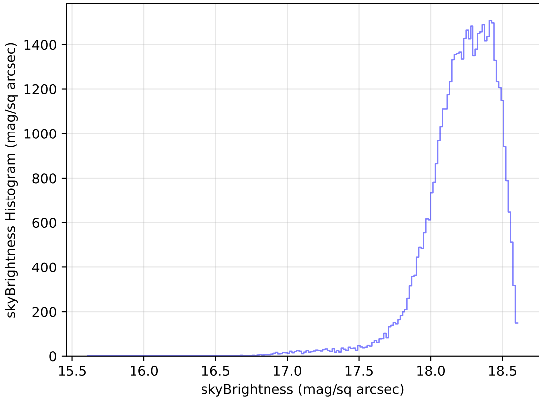
roll_pause_mjdp60_v3.4_10yrs Yr 1 y band: skyBrightness Histogram
