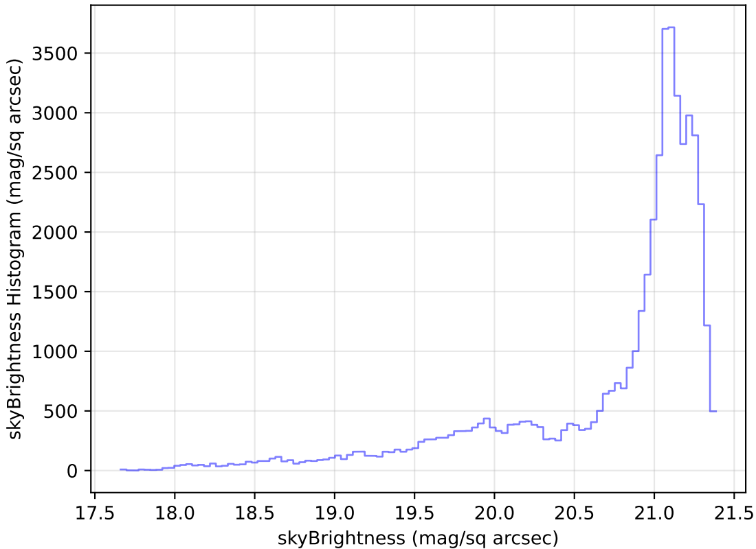
roll_pause_mjdp60_v3.4_10yrs Yr 1 r band: skyBrightness Histogram
