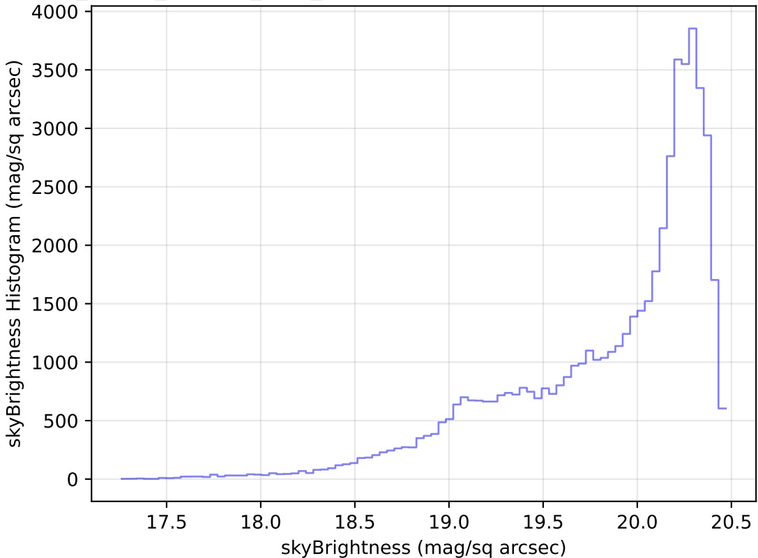
roll_pause_mjdp60_v3.4_10yrs Yr 1 i band: skyBrightness Histogram
