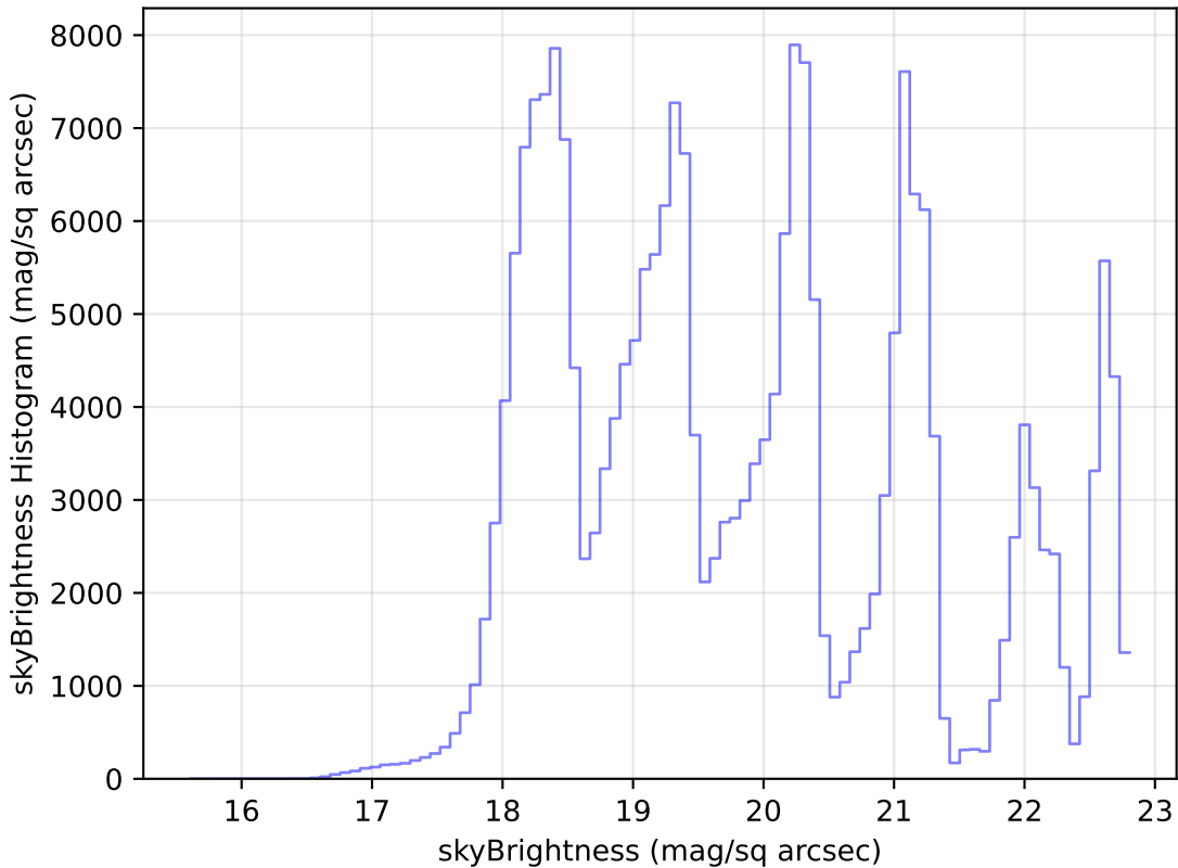
roll_pause_mjdp60_v3.4_10yrs Yr 1 all bands: skyBrightness Histogram
