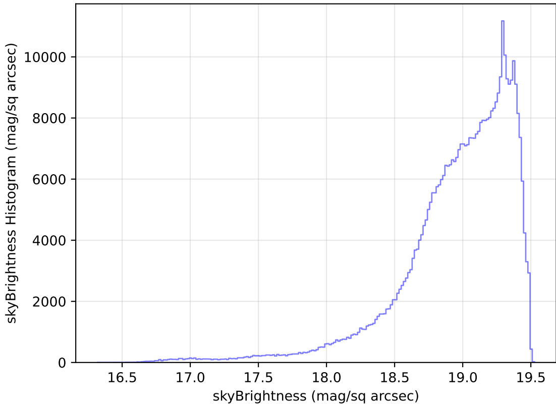
roll_pause_mjdp60_v3.4_10yrs WFD z band: skyBrightness Histogram
